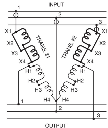
FIG. CC OPEN DELTA
